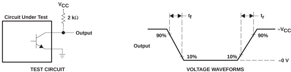
Figure 2. Switching Times
